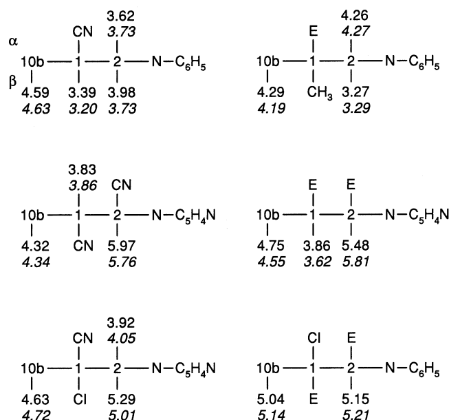
Scheme 1. Comparison of observed \delta_{\text{H}} values and those calculated with substituent increments (in italics) for the pyrazolidine protons of some cycloadducts; the horizontal line symbolizes the ring skeleton ( \text{E} = \text{CO}_2\text{CH}_3 )
